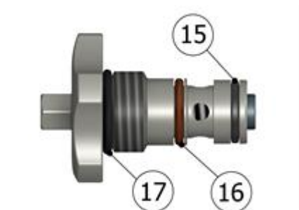
Figure 7. O-Rings Assembly Detail
